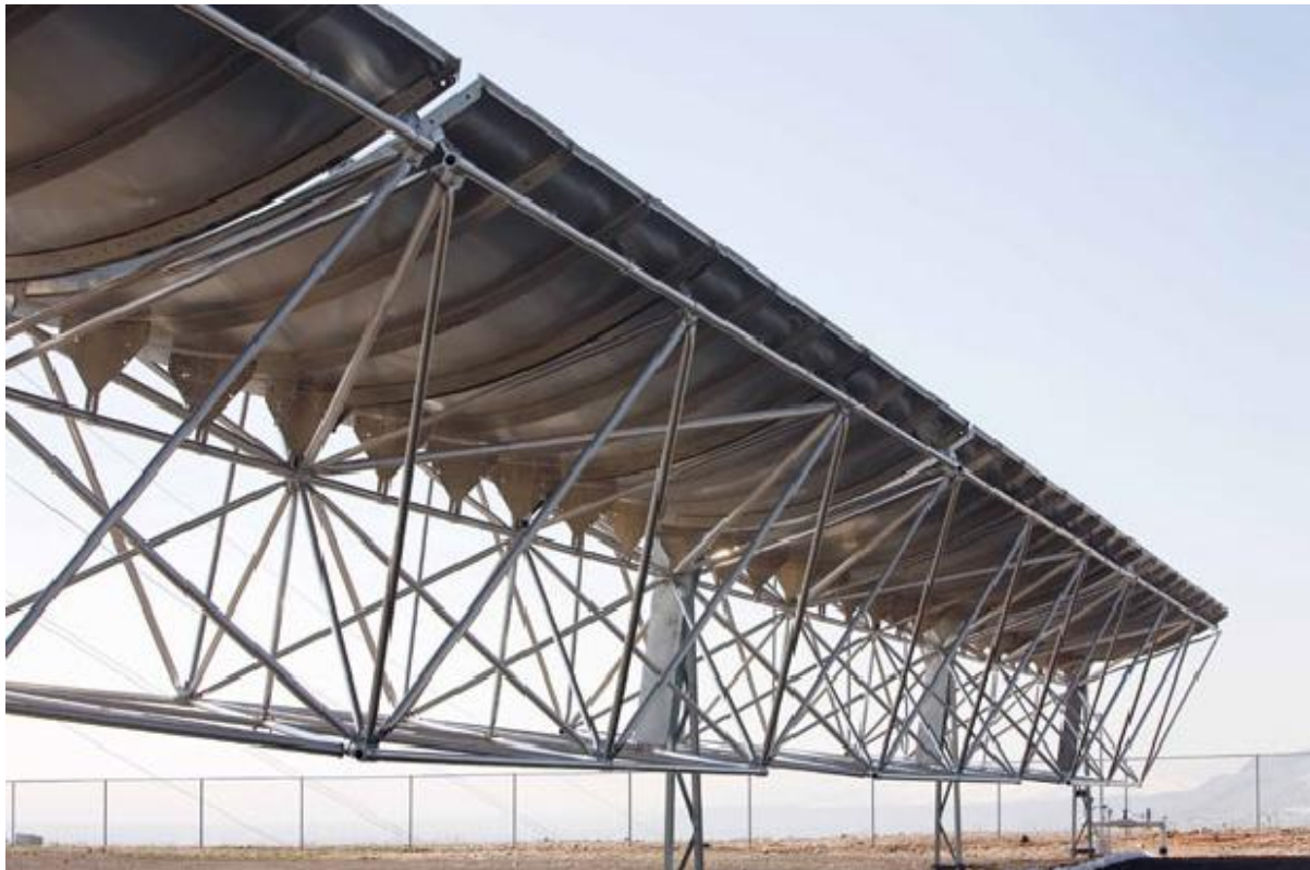
Figure 34: The Skytrough collector (source: Skyfuel)
