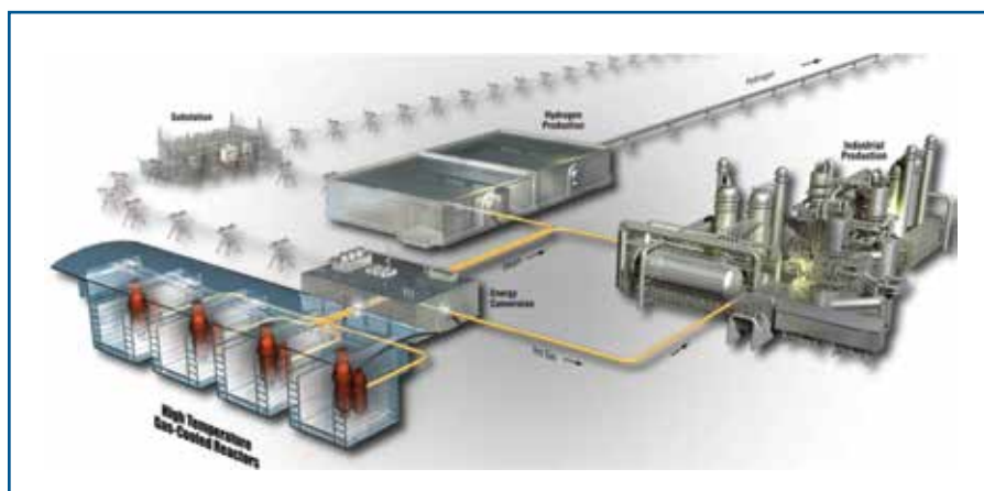
Fig. 10. Concept for large-scale centralized nuclear hydrogen production. 52
