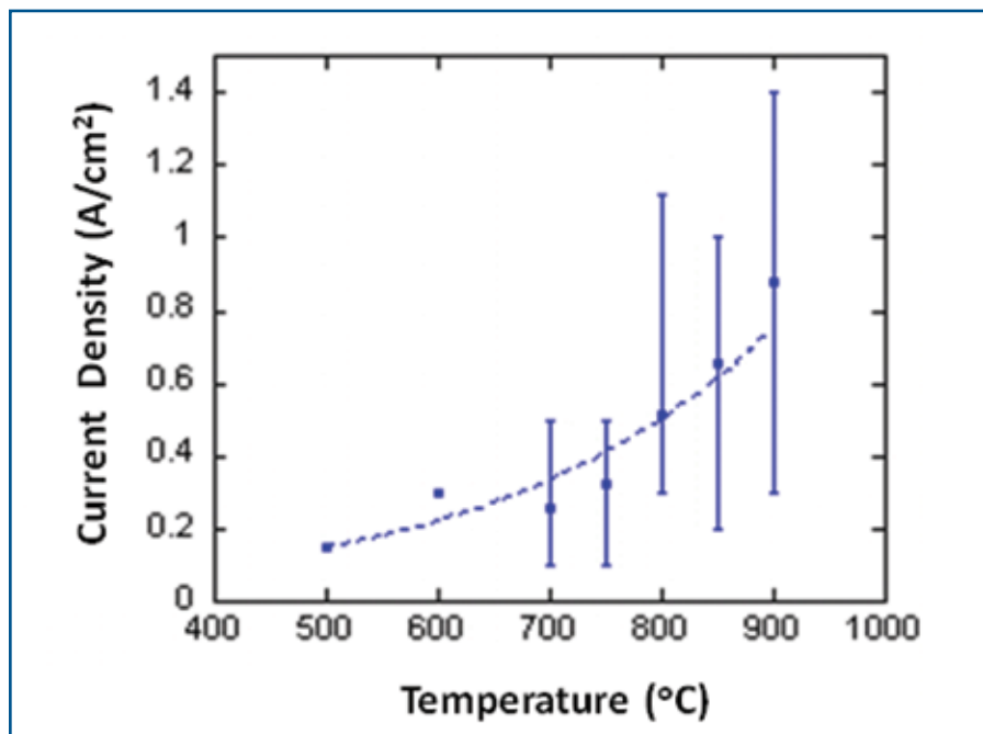
Fig. 8. Current densities at thermoneutral voltage reported for SOECs between 500° and 900°C (the bars show the range of values).
