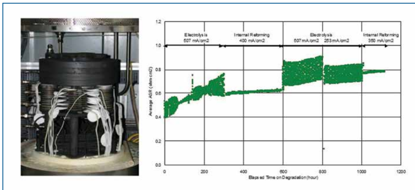
Fig. 12. Photograph of 10-cell stack (cell active area of 142 cm 2 ) and stack ASR in methane internal reforming fuel cell mode and steam electrolysis mode (fluctuations seen in steam electrolysis due to instability of steam generation and delivery). 16
