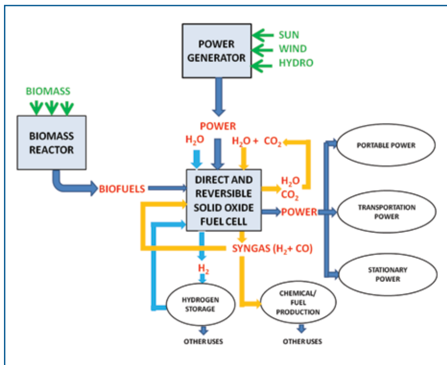
FIG. 3. An example of an RSOFC-based sustainable energy system.
