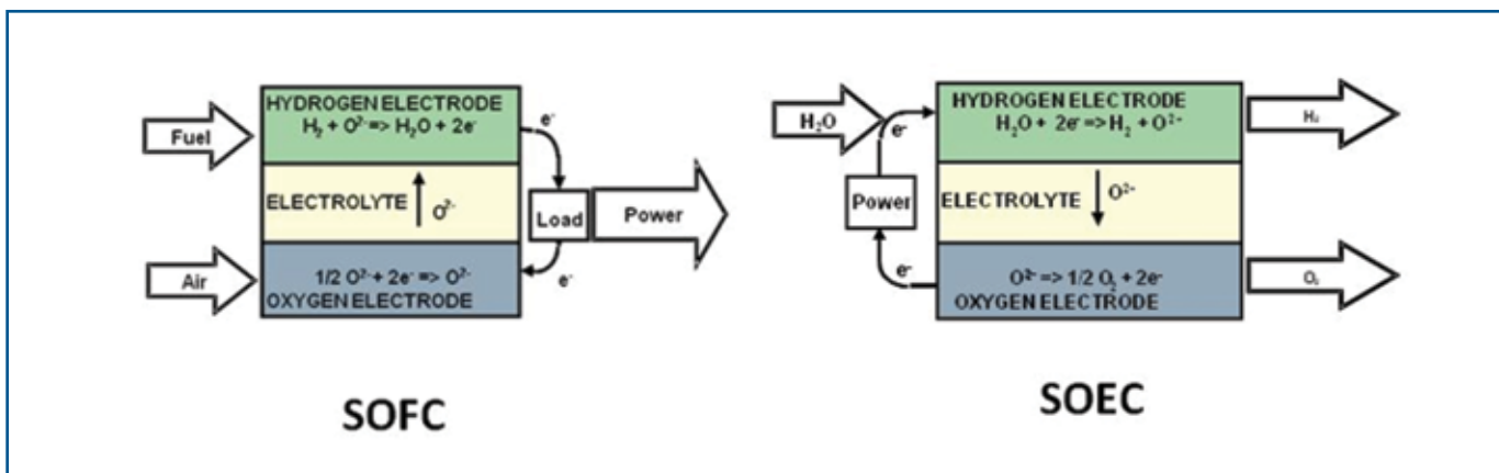
FIG. 1. Operating Principles of an RSOFC (written for hydrogen fuel in SOFC mode and steam electrolysis in SOEC mode).
