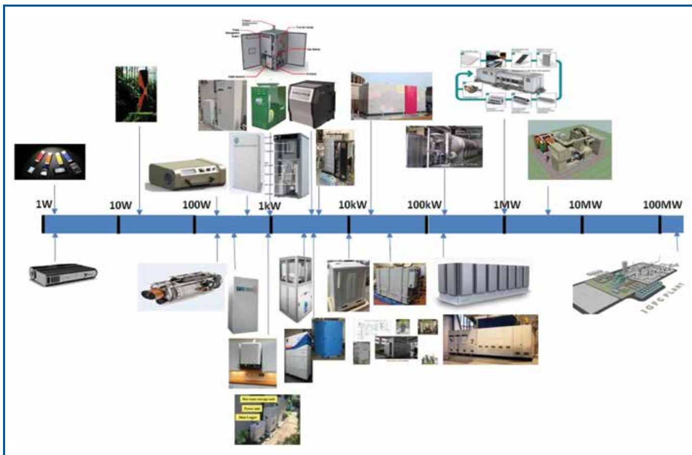
Fig. 4. SOFC power systems (hardware demonstrators, prototypes and pre-commercial systems up to 200 kW, concepts at 1MW and above).
