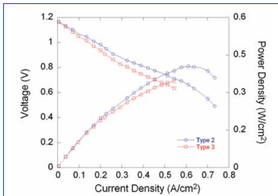
Fig. 6. Performance at 800°C with 7.3% ethanol balance He fuel and air oxidant for an anode-supported SOFC (with a dual layer anode consisting of a Cu-CeO 2 impregnated Ni/YSZ support outer layer and a Ni/YSZ electroactive inner layer). (Type 2 and 3 indicates different thermal treatments of infiltrated anodes). 28
