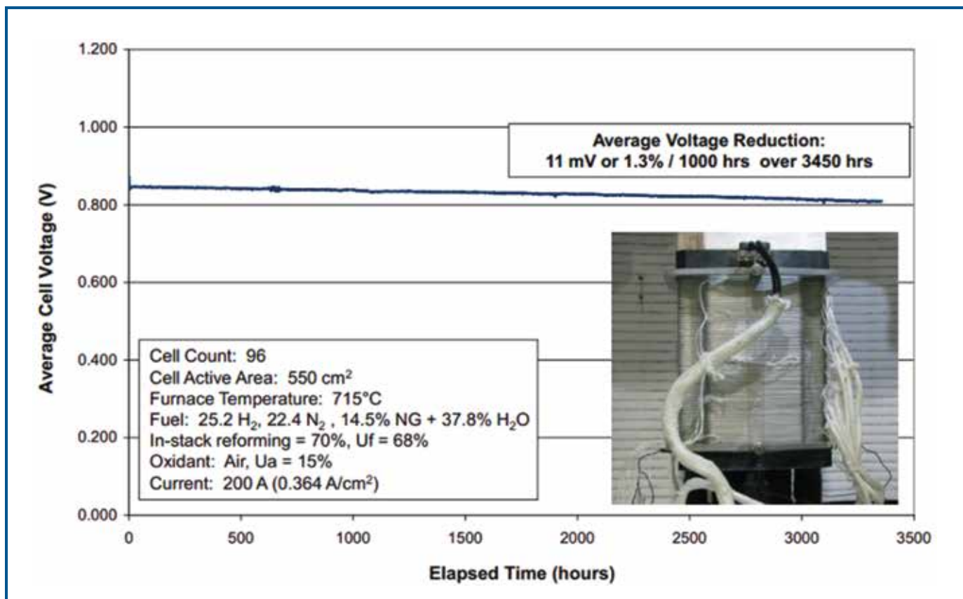
Fig. 7. Long-term performance of 96-cell planar stack. 9
