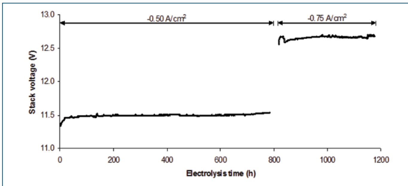
Fig. 9. Voltage as function of time for 1 kW 10-cell sStack of 12 cm x 12 cm footprint. Temperature = 850°C, gas input = 10% H 2 -45% H 2 O-45% CO 2 . 45
