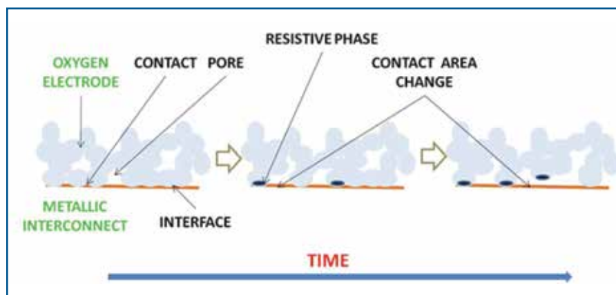
Fig. 5. Cathode (oxygen electrode)/metallic interconnect contact evolution.
