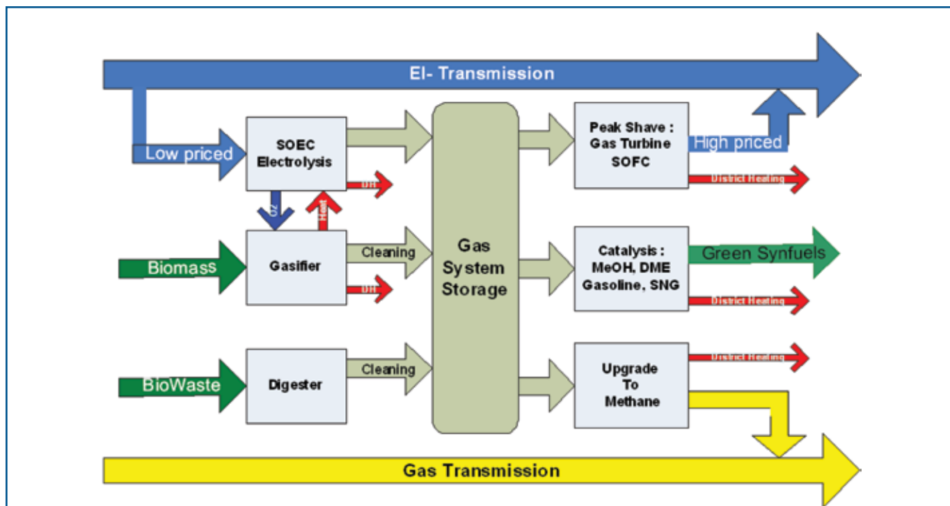
Fig. 11. Concept combining SOEC, biomass gasifier, and biomass digester. 53
